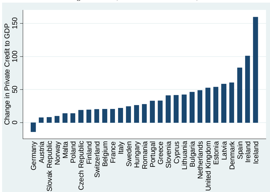
Figure 3: E30; Domestic Credit Growth, 2003-2008.
