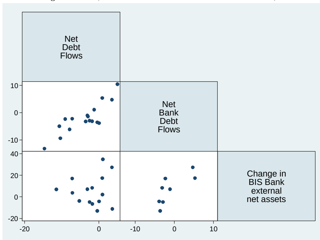
Figure 6: E30; International Debt Flows Alternative Measures, 2003-2008.
