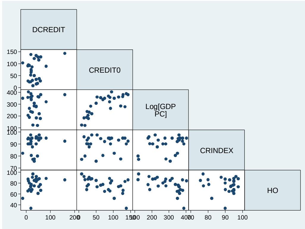
Figure 5: E30; Domestic Credit Growth and Country Characteristics, 2003-2008.
