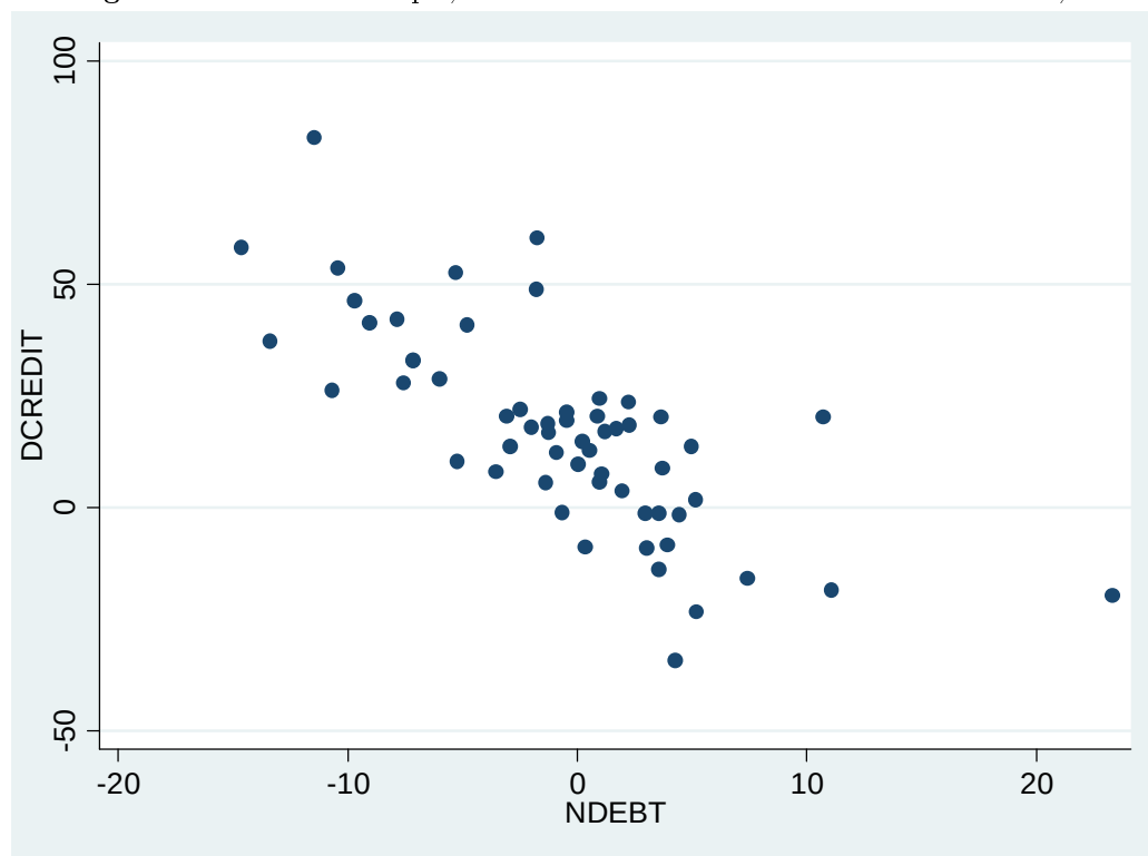
Figure 7: Extended Sample; Domestic Credit Growth and Net Debt Flows, 2003-2008.
