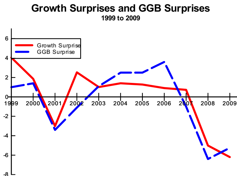
Figure 1: Growth Surprises and GGB Surprises, 1999 to 2009.
