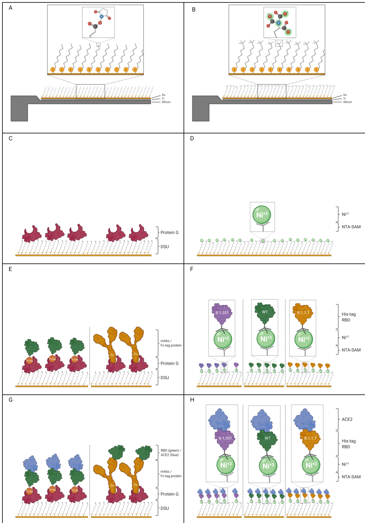
Fig. S1 Protein G/Fc-tag and NTA/His-tag functionalization process. Each cantilever used in the present study is coated with 3 nm of Titanium and 23/33 nm of Gold (top and bottom side, respectively) via metal evaporation (in A , B only the top side coating is shown in order to facilitate a simplified graphical representation). A Incubation of the sensitive surface in
