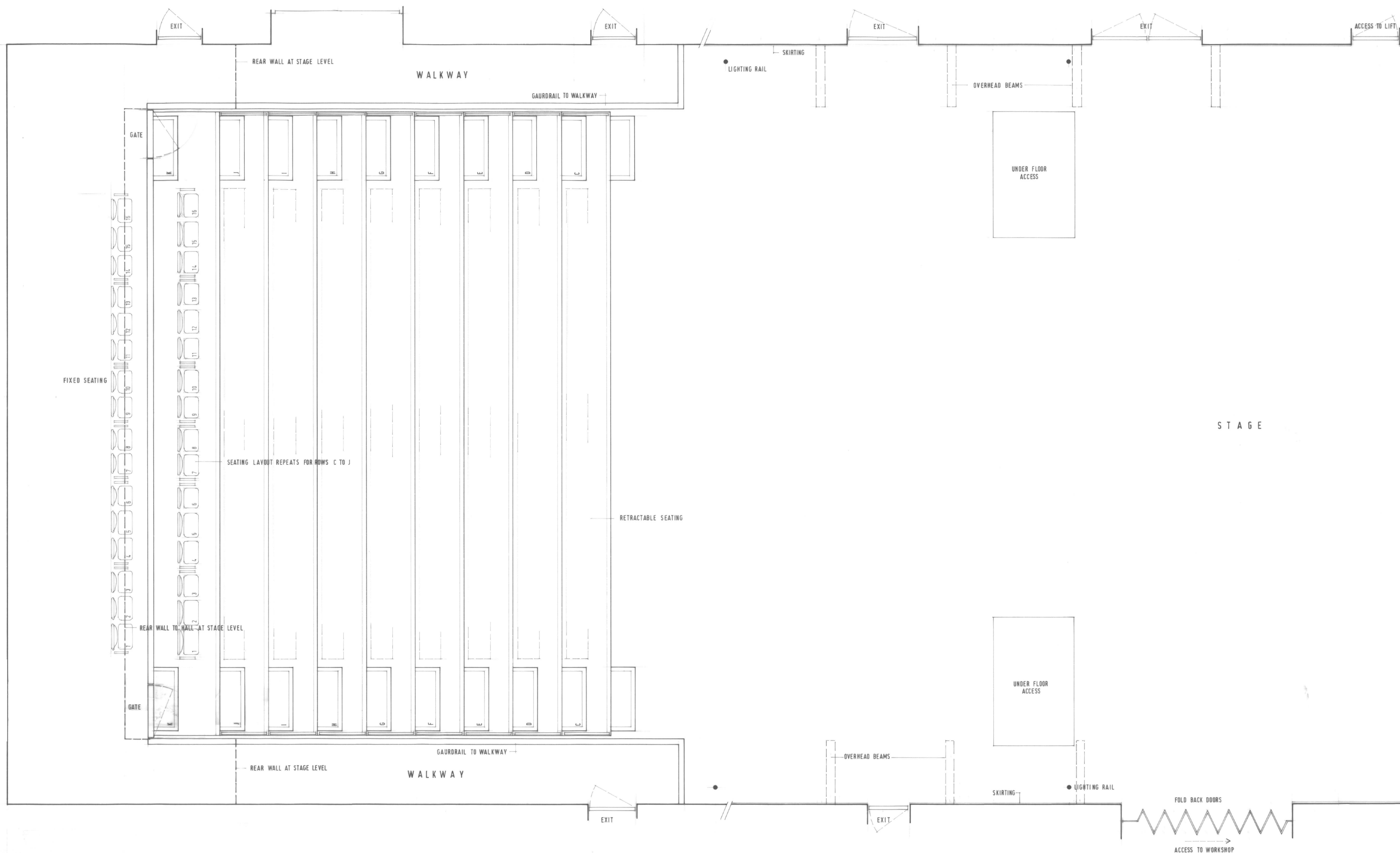
PLAN ON WALKWAY / STAGE THE SAMUEL BECKETT STUDIO THEATRE Drg. No. 01 1:25
