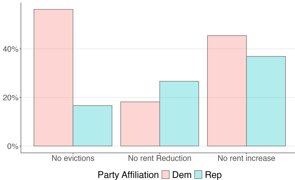
Figure 5: Judge decisions
