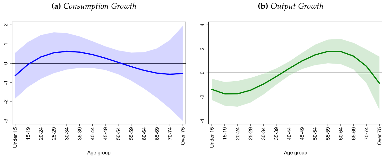
Fig. 4. Implied coefficients on five-year population share growth rates: consumption and output growth.
