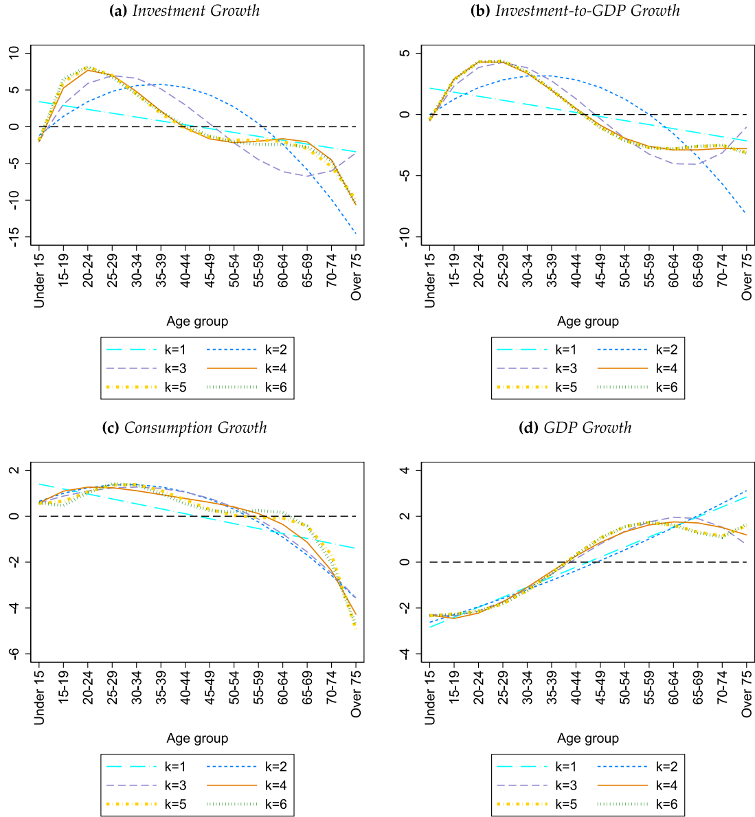
Fig. 9. Age coefficients: Changing polynomial order.
