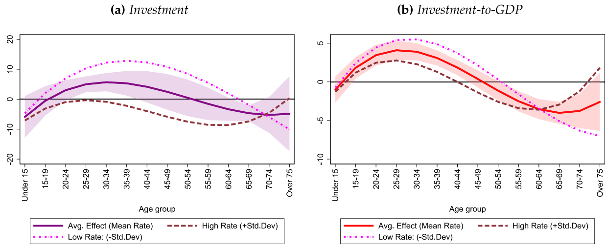
Fig. 3. Conditional interest rate impacts on age structure coefficients.
