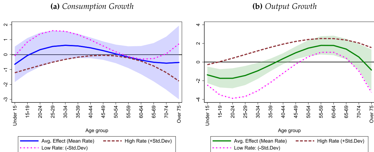
Fig. 5. Conditional interest rate impacts on age structure coefficients.
