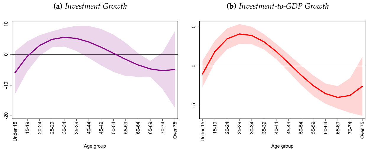
Fig. 2. Implied coefficients on five-year population share growth rates: Investment growth.
