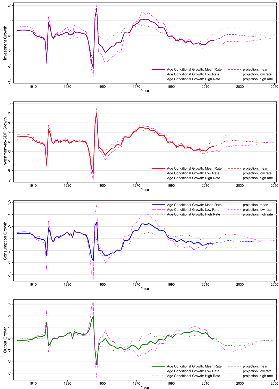
Fig. 6. Predicted impact of age structure: United States.
