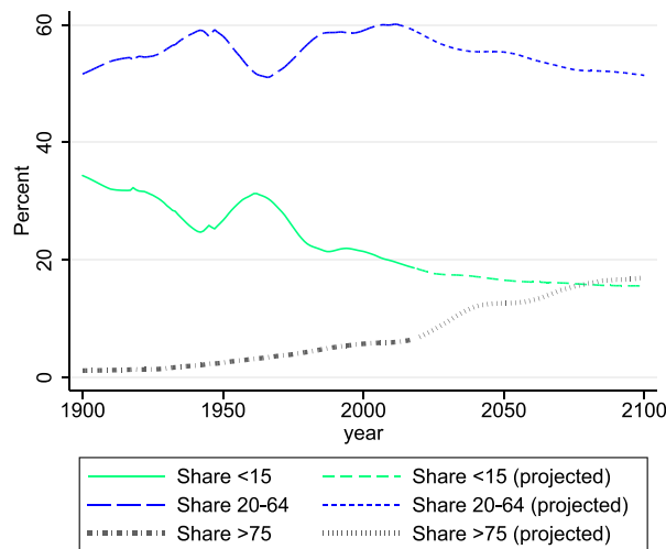
Fig. 1. Variation in population data: United States.
