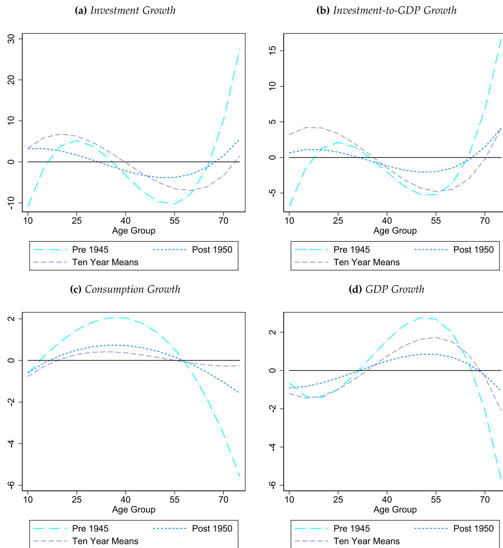
Fig. 10. Age coefficients: Various samples.
