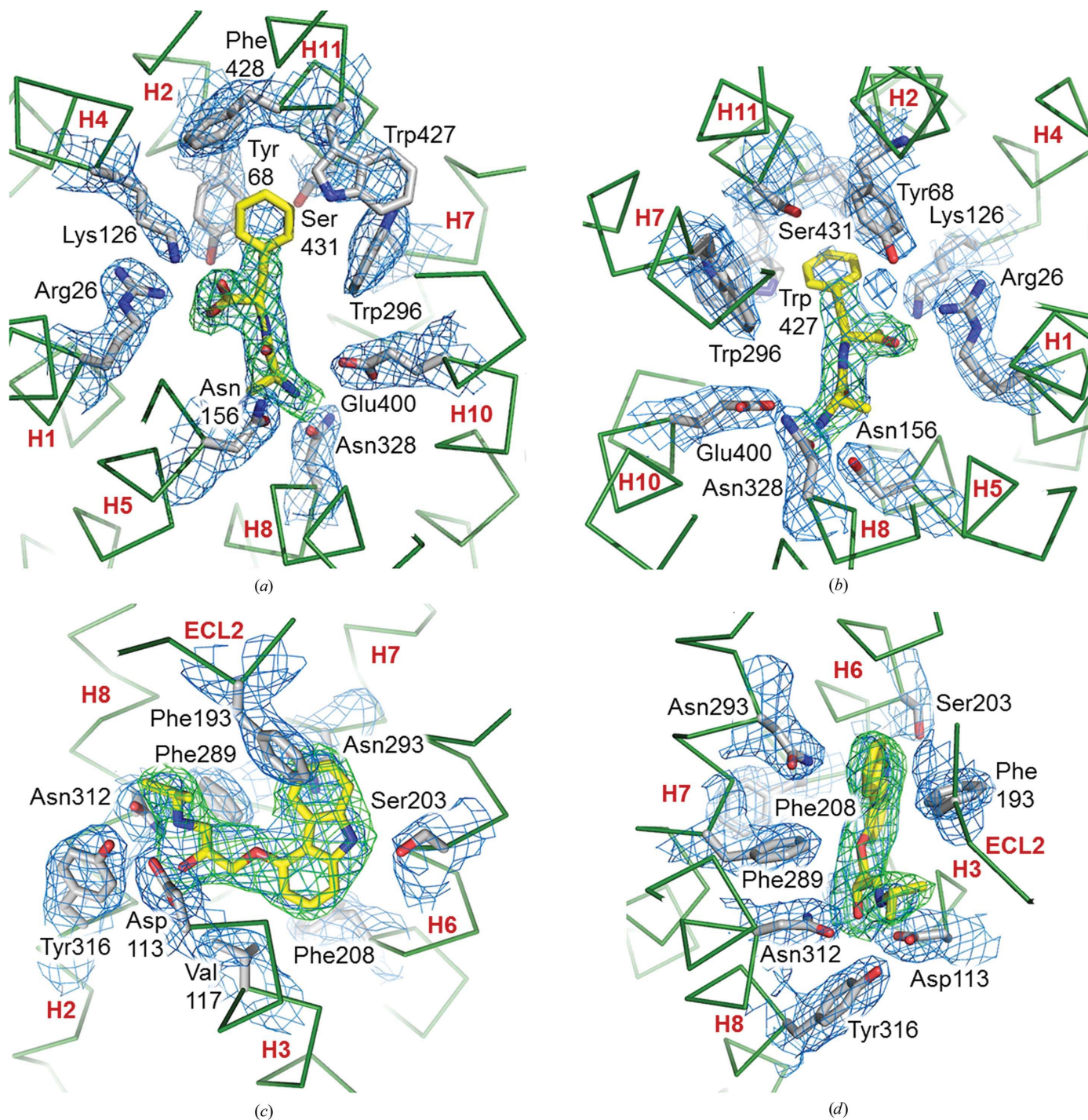
Figure 4 Electron-density maps of ligands bound to PepT S and \beta_2 AR in crystal structures solved by the IMISXcryo method at resolutions of 2.4 and 2.5 Å, respectively. (a, b) Views into the peptide-binding pocket of PepT S reveal the dipeptide Ala-Phe in well defined density. (c, d) Views into the ligand-binding pocket of \beta_2 AR reveal the partial inverse agonist carazolol in well defined density. Ligands are shown with yellow C atoms and with an F_o - F_c map (green mesh) contoured at 3\sigma . 2F_o - F_c maps are contoured at 1\sigma (blue mesh). Relevant residues are highlighted as sticks with grey C atoms. The protein backbone is shown in thin ribbon representation coloured green. Helices (H) and an extracellular loop (ECL) are indicated following the notation in the original literature. Stick models include N (blue) and O (red) atoms.
