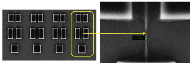
Example of a fabricated structure with a 50 nm (approx.) channel.
