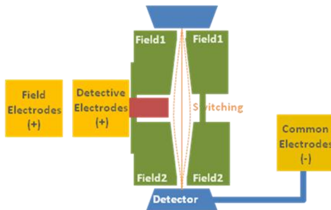
Illustration of side view of NEMS device.
